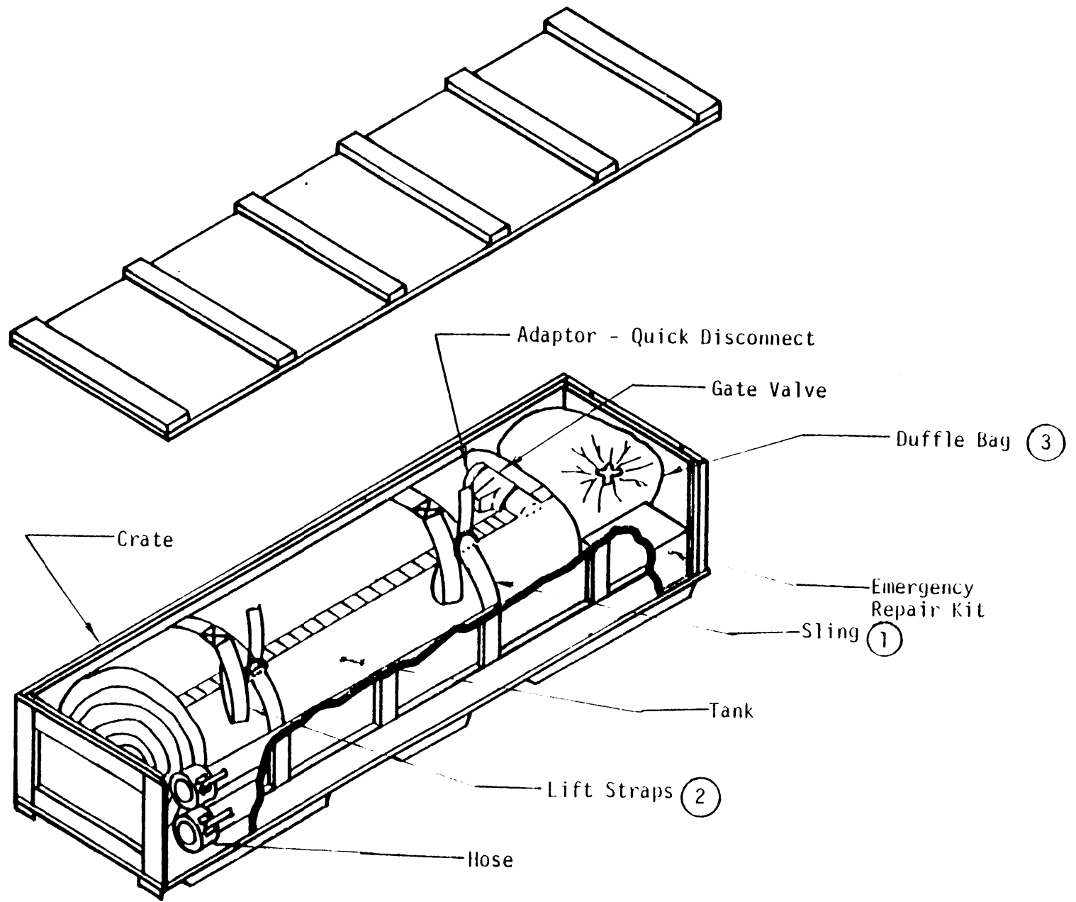
CRATED ASSEMBLY
