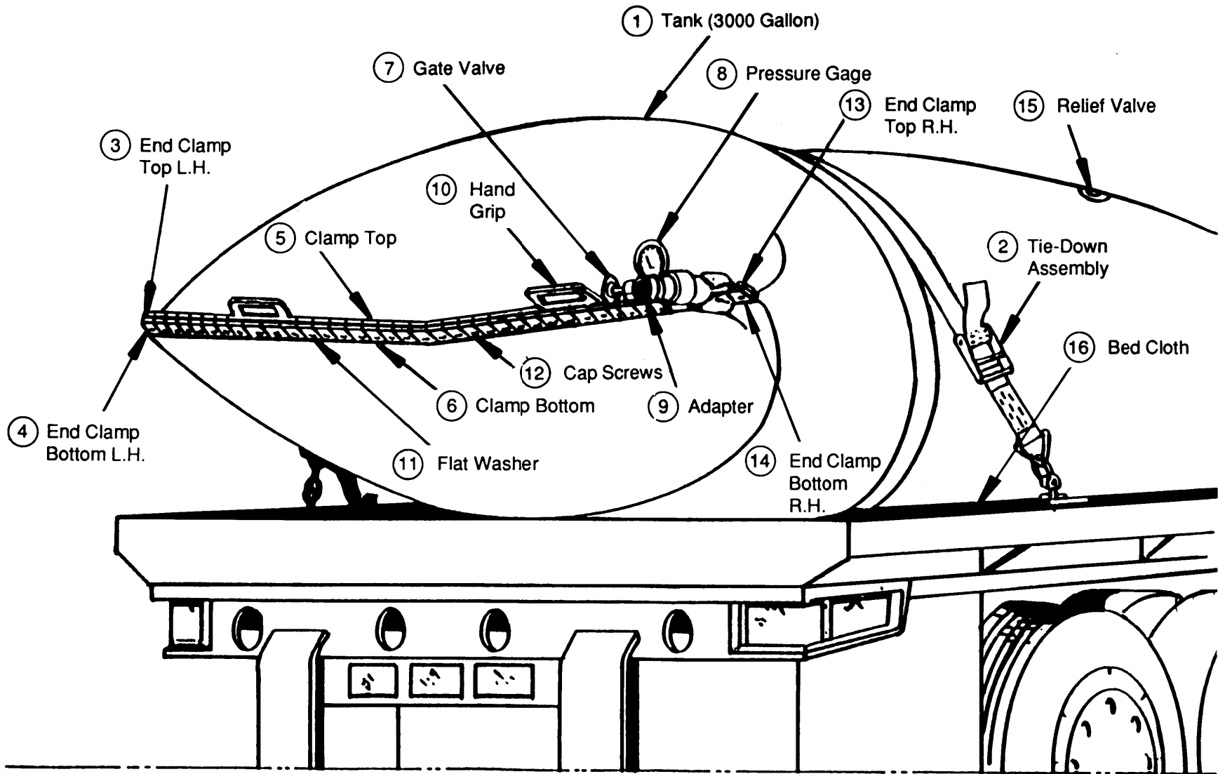
TANK WITH HARDWARE AND TIE-DOWN ASSEMBLY (Model 91093)
