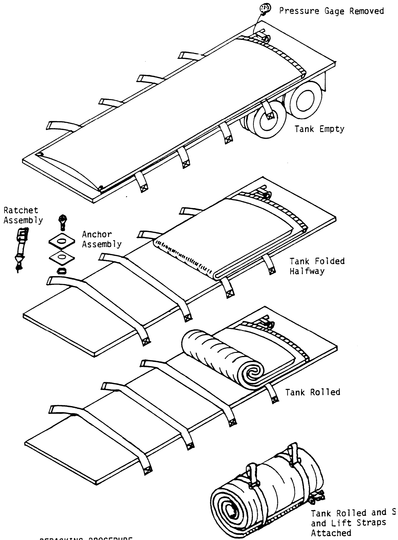
REPACKING PROCEDURE FIGURE 2-8
