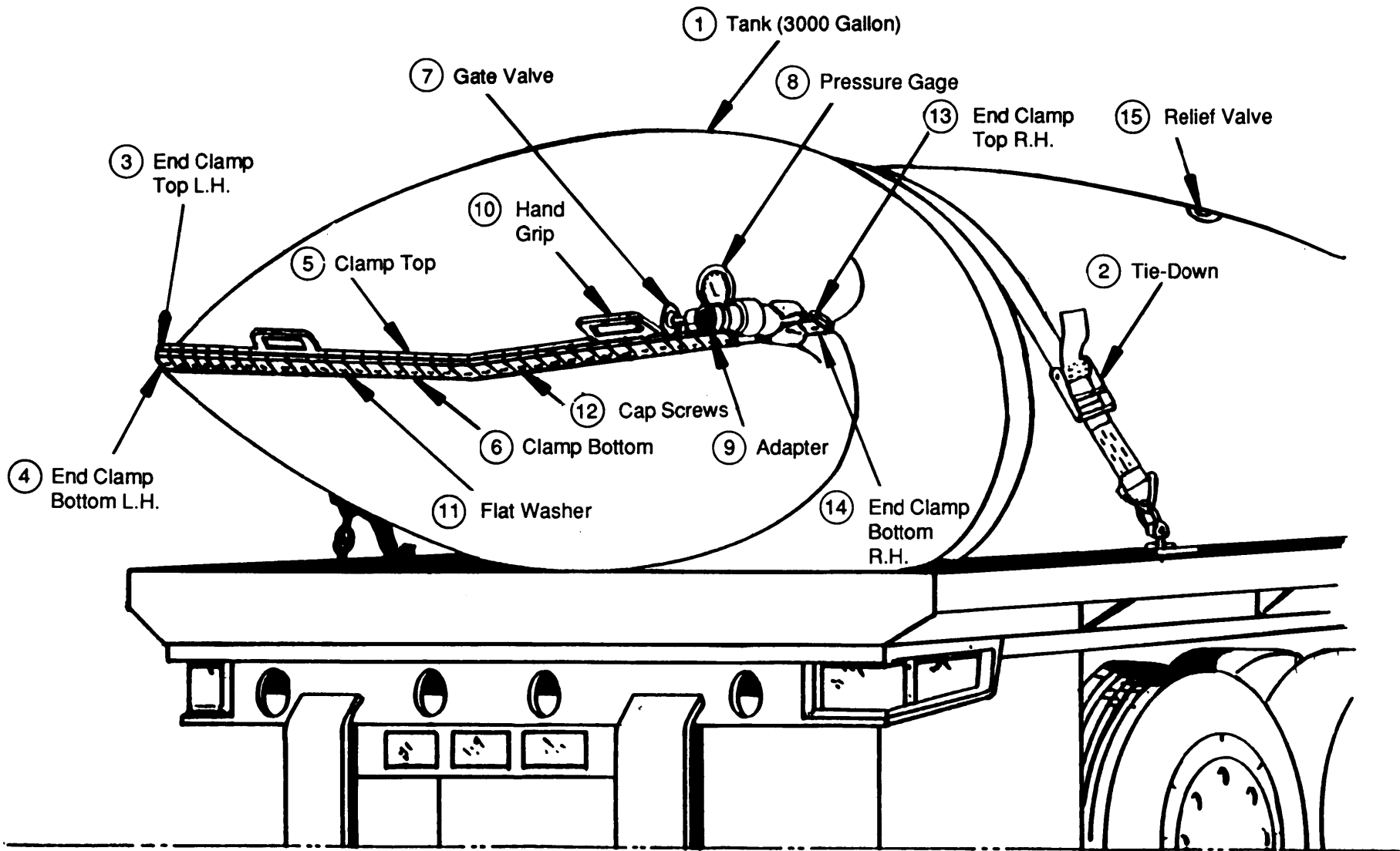
TANK WITH HARDWARE AND TIE-DOWN ASSEMBLY (MODEL 3,000 gallon )
