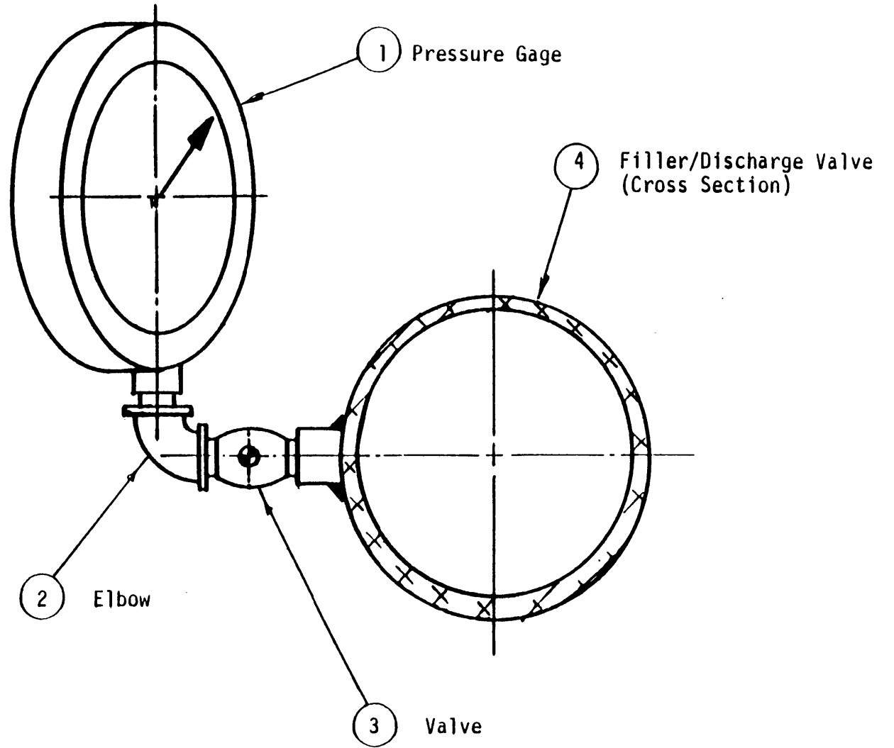
PRESSURE GAGE ASSEMBLY
