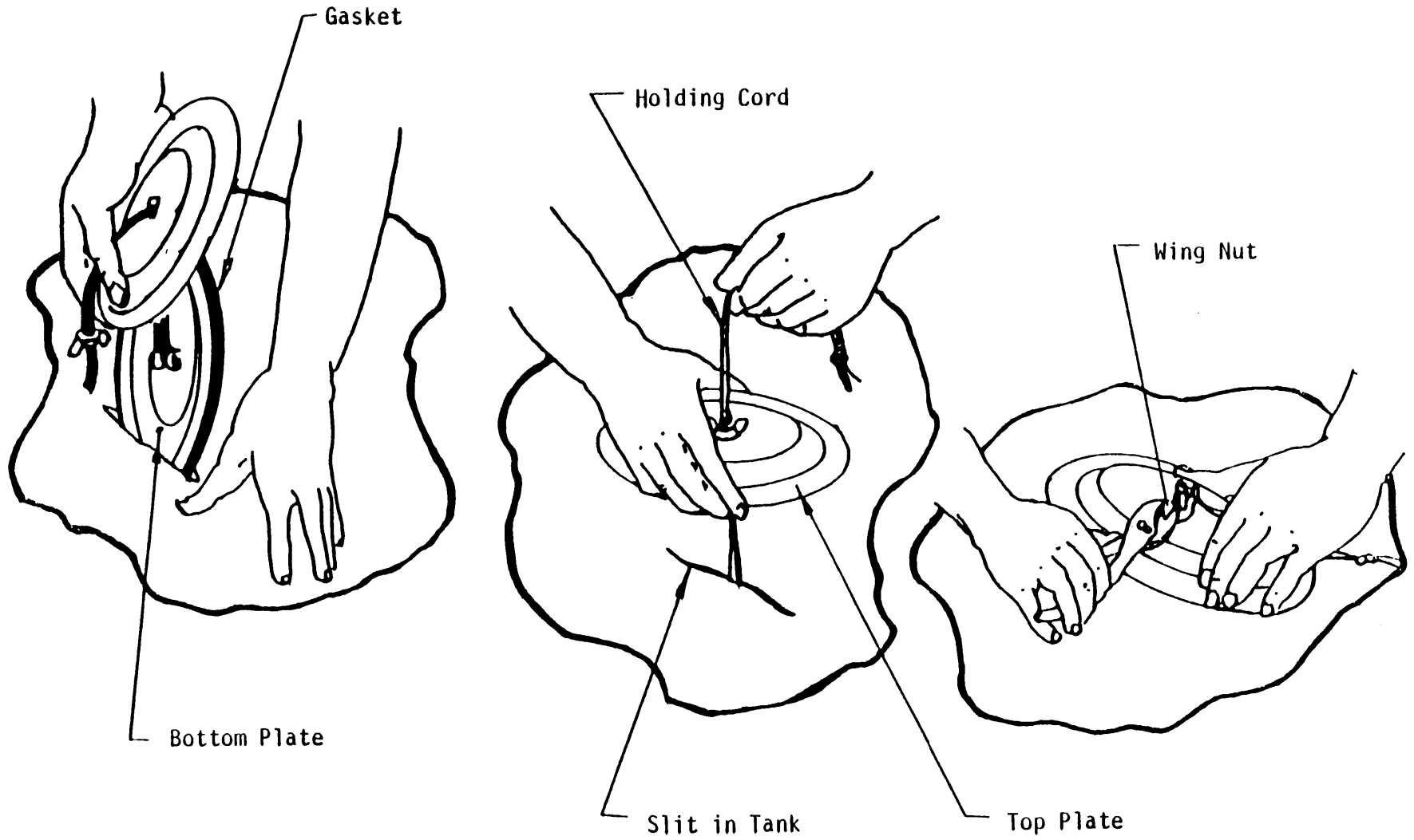
INSTALLATION OF SEALING CLAMPS
